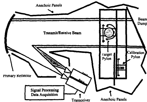
Fig. 1. Typical compact-range room configuration.
