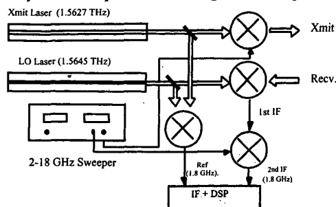
Fig. 4. Simplified diagram of 1.56 THz Laser Transceiver.
