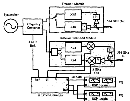
Fig. 2. The 524 GHz transceiver block diagram.
